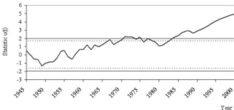
Figure 10 - Mann-Kendall sequential test applied to Apparent Temperature
