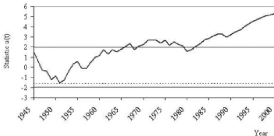
Figure 9 - Mann-Kendall sequential test applied to Discomfort Index
