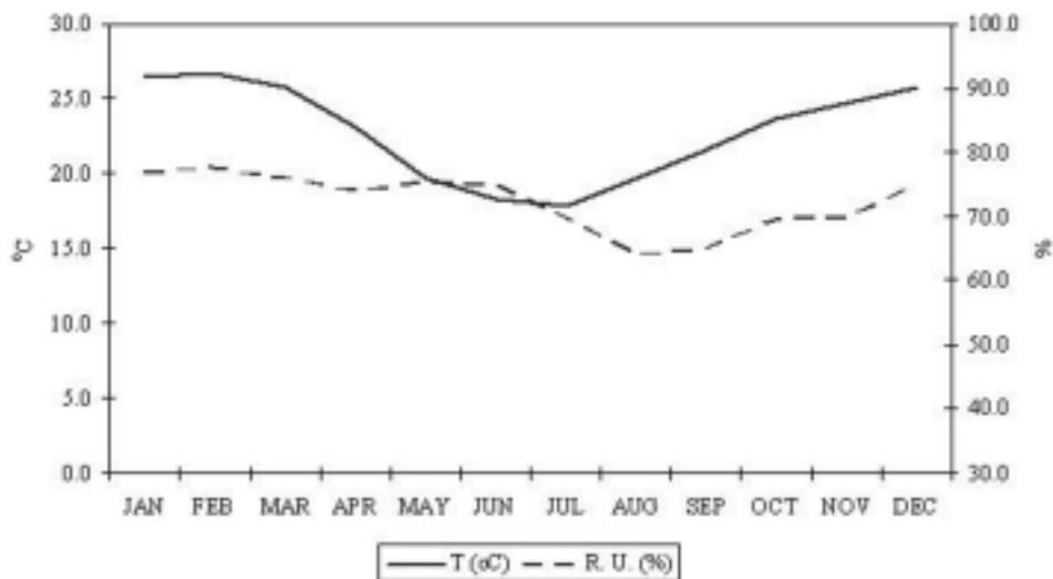
Figure 7 - Chart showing the seasonality of the average monthly temperature and monthly relative humidity
