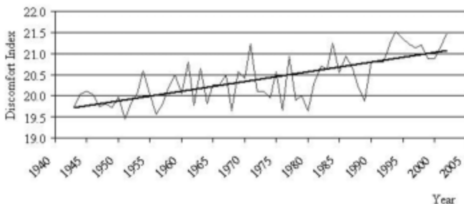
Figure 8 - Temporal evolution of the annual values of the Discomfort Index and the trend line generated
