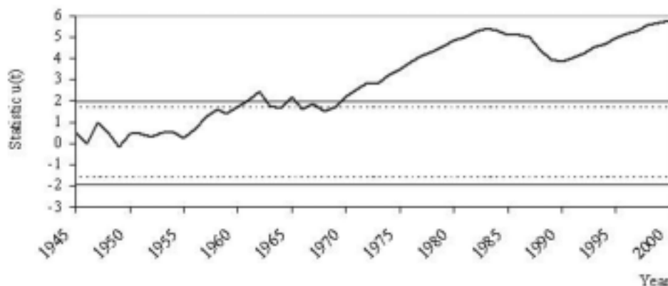
Figure 11 - Mann-Kendall sequential test applied to Relative Humidity
